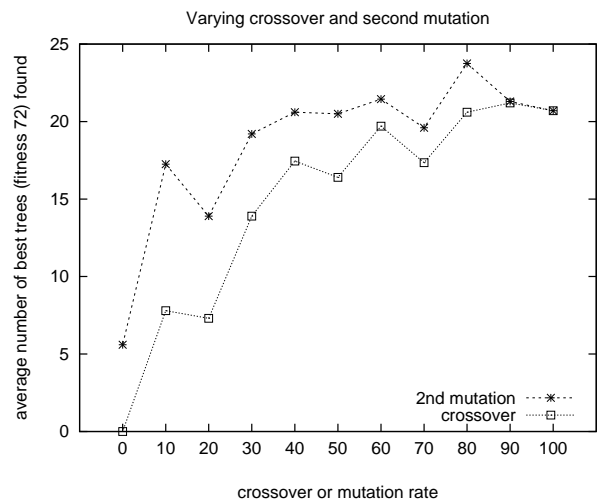
Figure 6: The effects of varying crossover rate while holding second mutation constant and of varying the second mutation rate while holding the crossover rate constant. The average number of best trees (45 max) found by each parameter setting is illustrated.
