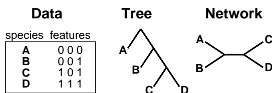
Figure 1: A toy example data set, sample phylogeny, and sample network. In this example, there are four species and three features. The tree formed shows the hypothesis that species B is related to species A, gaining the third feature. Similarly, C and D are more closely related to B than to A, also acquiring new features.
