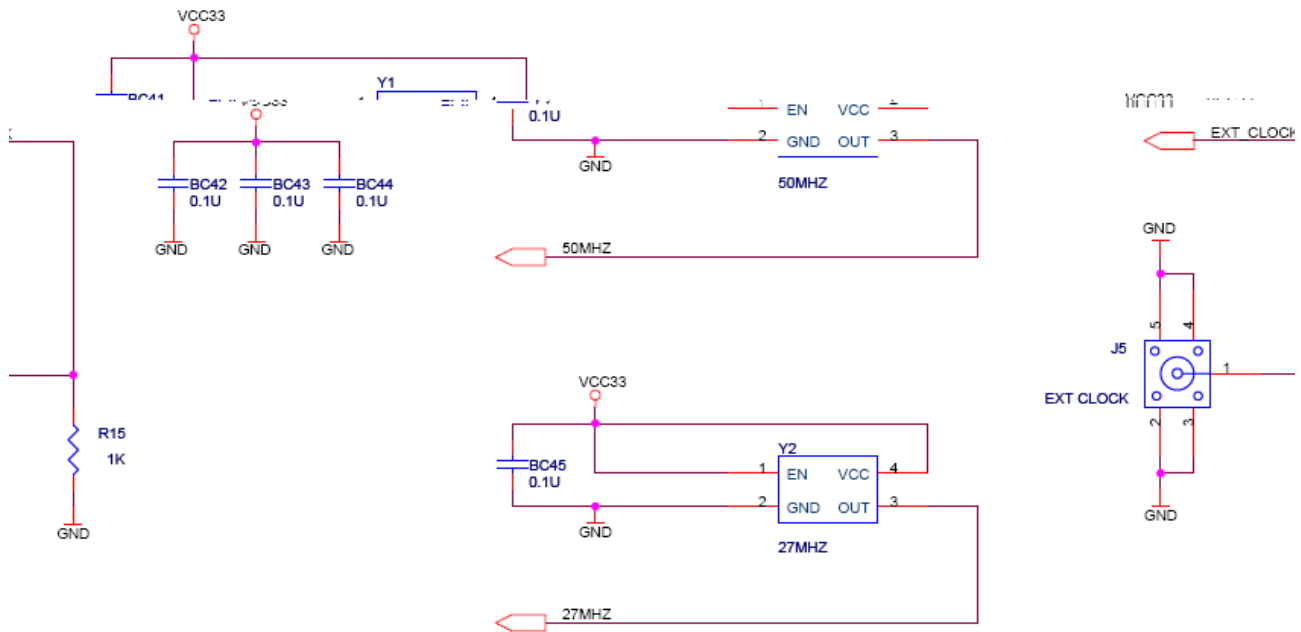
Figure 4.8. Schematic diagram of the clock circuit.
