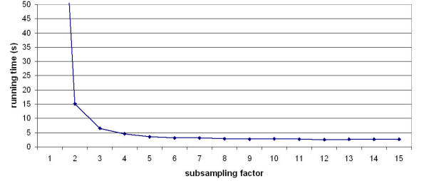
Figure 13: Speed-up due to downsampling for 17 segments and a 576x768 image. The value for the full-scale filtering is 173 sec.
