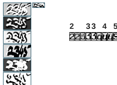
Fig. 24. A Graph Transformer pulls out the best interpretation from the output of the SDNN.
