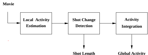
Figure 1: Steps performed for the computation the activity/duration features.
