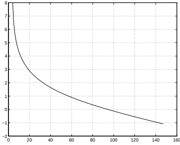
Figure 2: Shot detection threshold for a Weibull prior.
